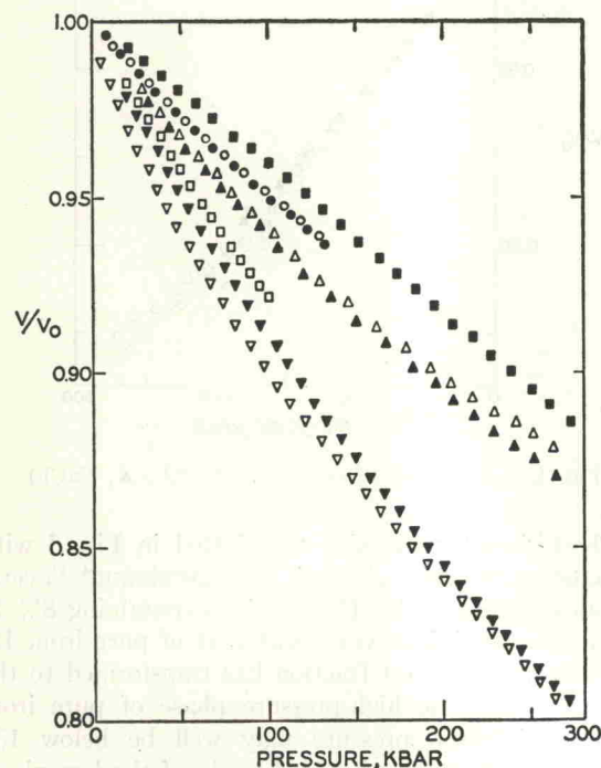
Fig. 3. V/V_0 vs pressure for iron and alloys. ○, Fe; ●, Fe+8.0% Si; ■, \text{Fe}_3\text{Si} ; □, Si (Bridgman); △, FeAl; ▲, \text{Fe}_3\text{Al} ; ▼, AgMg; ▽, Al (shock data).
