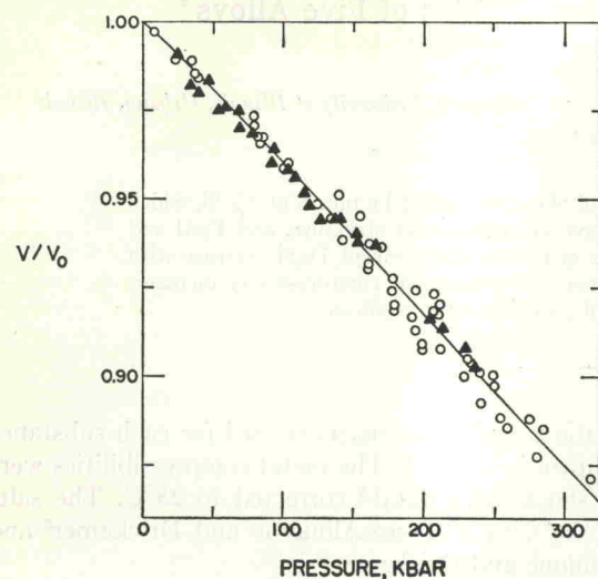
Fig. 2. V/V_0 vs pressure— \text{Fe}_3\text{Si} . (○, Nb; ▲, NaF.)
