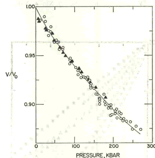
FIG. 1. V/V_0 vs pressure—Fe 3 Al. (O, Nb; ▲, NaCl.)
